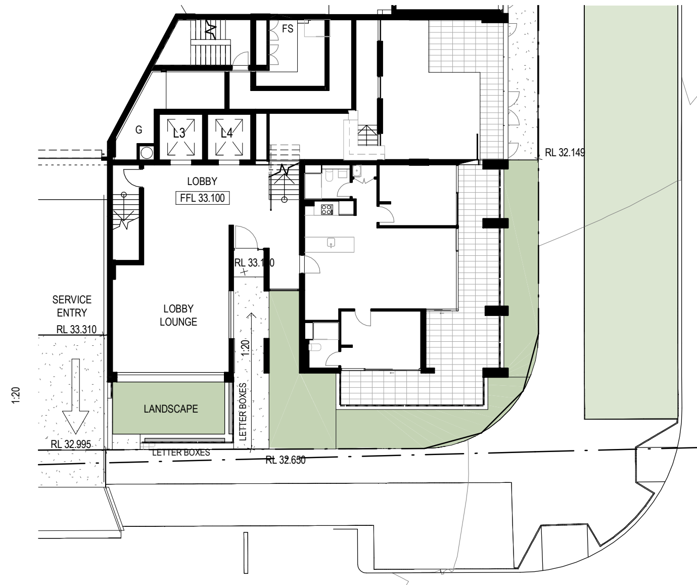
1 LEVEL 01 PLAN
